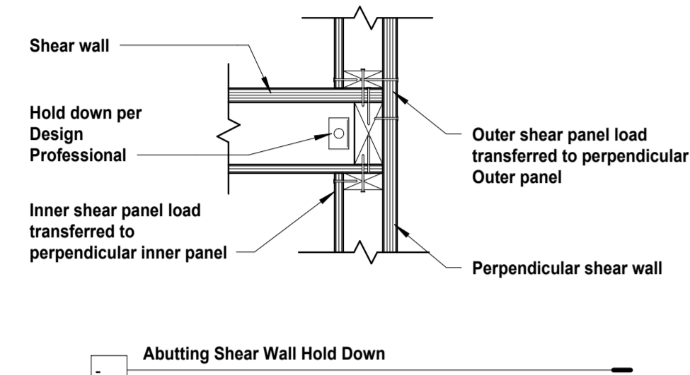
1 Abutting Hold downs 1" = 1'-0"
