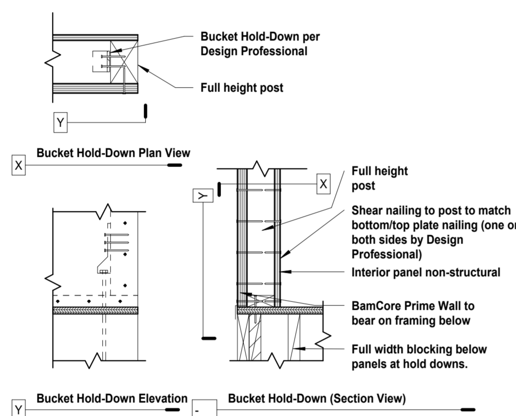
7 Bucket Hold-Down to BamCore Panel 1" = 1'-0"
