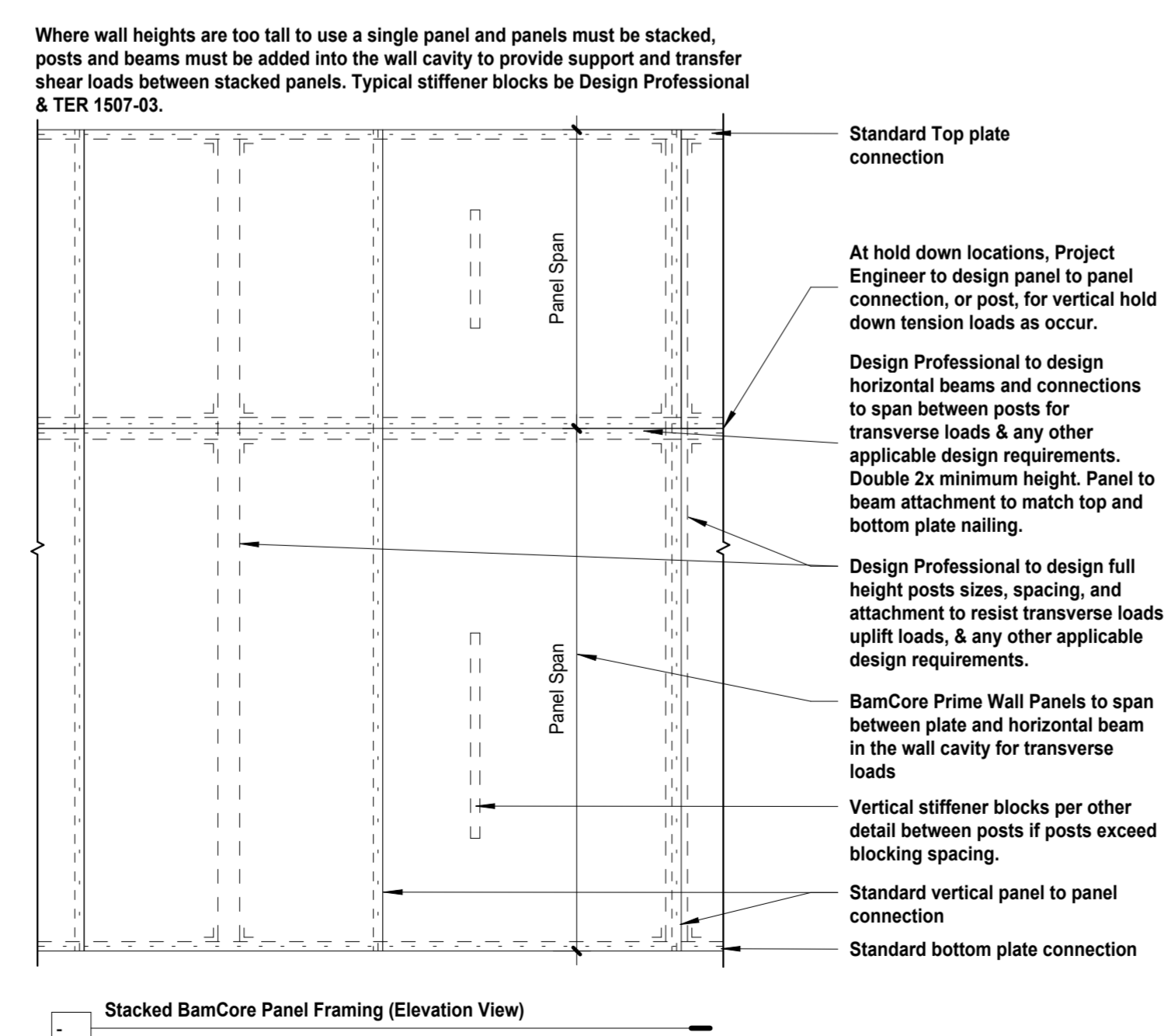
10 Tall Wall Framing 1/2" = 1'-0"
